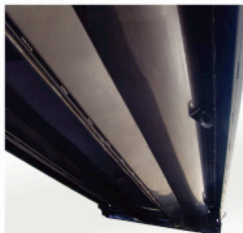
Above is the 600T's crossmemberless understructure and formed long sills with rubber cushion.
